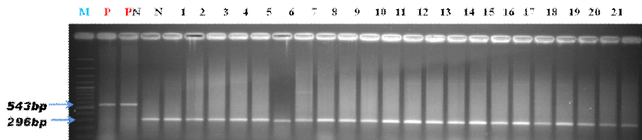
Fig. 1: Gel pictures depicting co-dominant PCR assays for crtRB1-3' TE polymorphism among the maize inbreds
