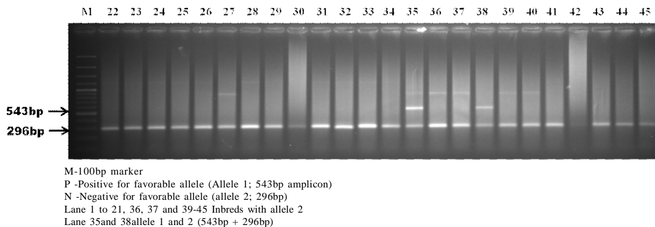
Fig. 2: Gel pictures depicting co-dominant PCR assays for crtRB1-3' TE polymorphism among the maize inbreds (allele type 1 and 2)
