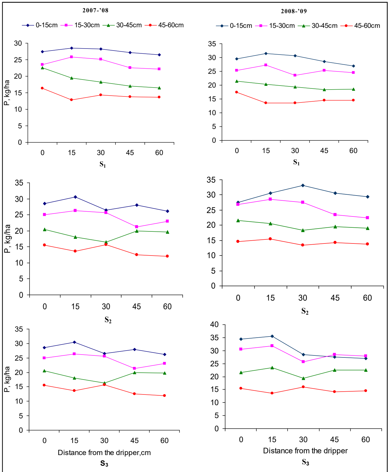
Fig. 1: Phosphorus ( P, \text{kg ha}^{-1} ) distribution as influenced by drip irrigation at 0.6 ET with different salinity levels
