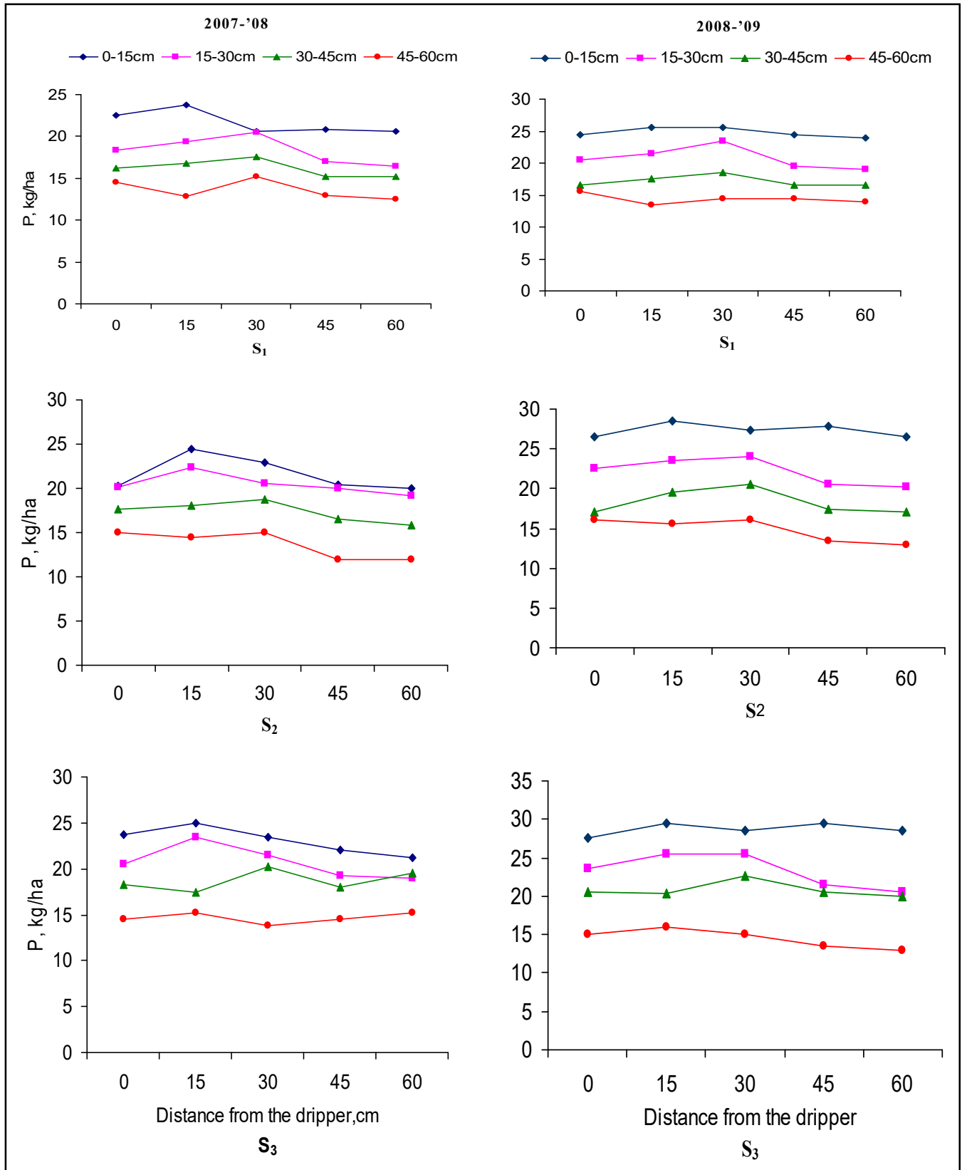
Fig. 4 : Phosphorus (K, kg ha -1 ) distribution as influenced by drip irrigation at 1.2 ET with different salinity levels
